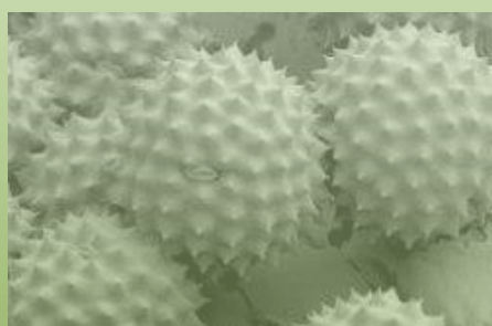
Ragweed pollens and score-symptom in France (2010-2012)
